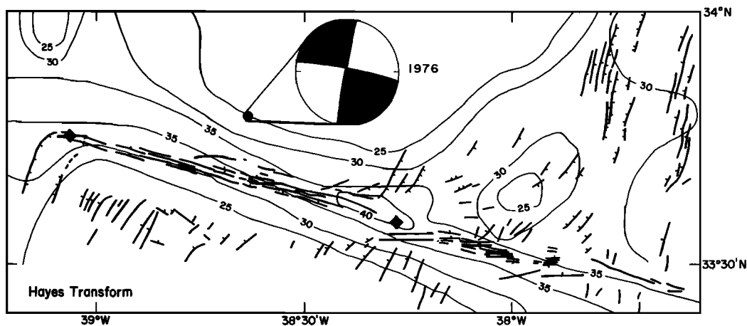
Fig. 4. Bathymetry and tectonic lineations of the Hayes transform. Bathymetric contours, in hundreds of meters at 500-m intervals, are from Feden et al. [1975]. Tectonic lineations (heavy lines), inferred from a GLORIA side scan sonar survey, are from R. C. Searle (personal communication, 1986); barbed lines indicate normal faults (barb on the down-thrown side). The inferred positions of the RTIs are indicated by solid diamonds. Also shown are the ISC epicenter (probably mislocated by 10 km to the north) of the earthquake of March 28, 1976, and the focal mechanism determined in this study by body waveform inversion.
