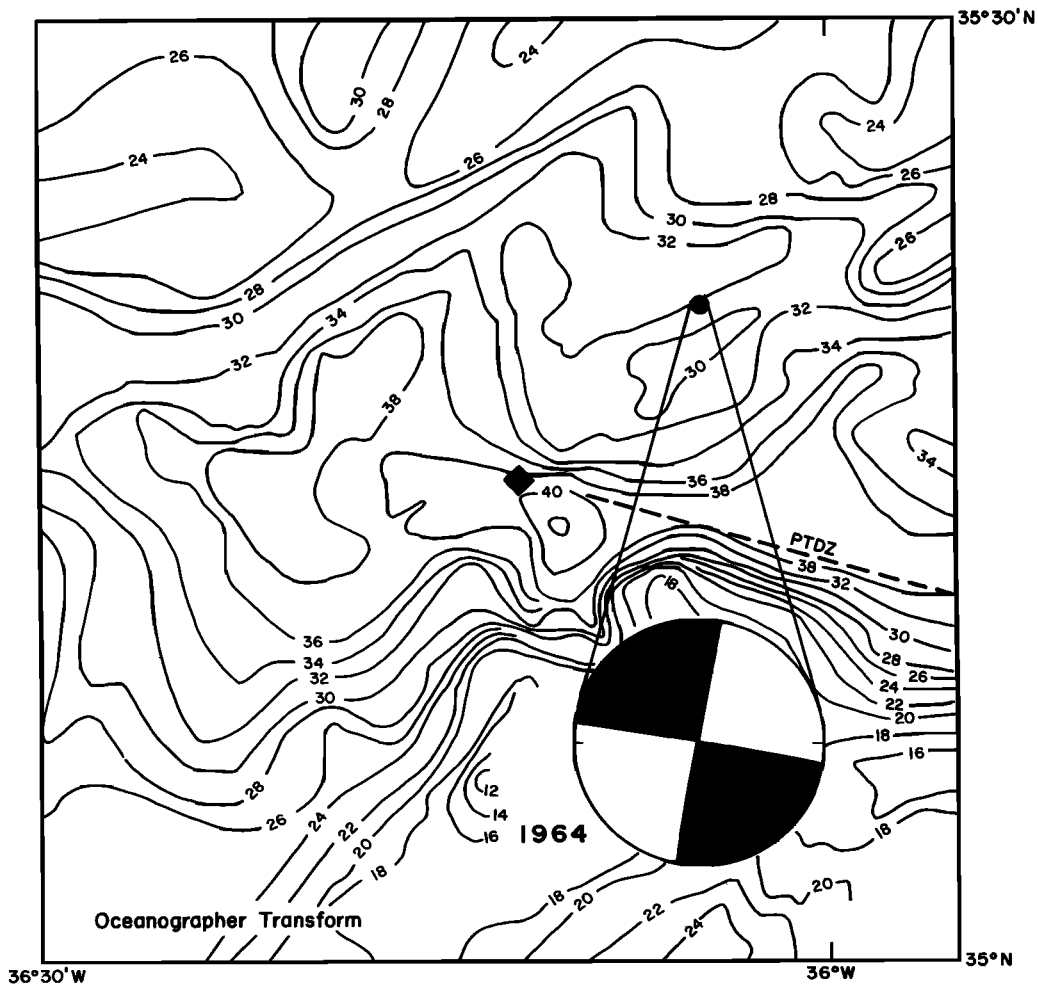
Fig. 3. Bathymetry of the western end of the Oceanographer transform. Bathymetric contours, in hundreds of meters at 200-m intervals, are from Williams et al. [1984]. The positions of the RTI (solid diamond) and the PTDZ are from Williams et al. [1984]. Also shown are the focal mechanism, determined by body waveform inversion, and the ISC epicenter (probably mislocated by 10–15 km to the north) for the earthquake of May 17, 1964.
