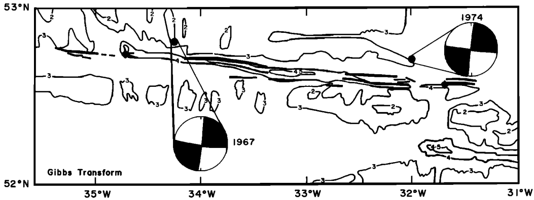
Fig. 2. Bathymetry, tectonic lineations, and locations and mechanisms of large earthquakes on the western segment of the Gibbs transform. The epicenters of the earthquakes of February 13, 1967, and October 16, 1974, are from the ISC and are probably mislocated by 10–15 km to the north (see text). The focal mechanisms determined in this study by body waveform inversion are shown as equal-area projections of the lower focal hemisphere; compressional quadrants are shaded. Major transform-parallel tectonic lineations (heavy lines), identified from GLORIA side scan sonar images, and bathymetric contours, in kilometers, are from Searle [1981]. Ridge-transform intersections are indicated by solid diamonds.
