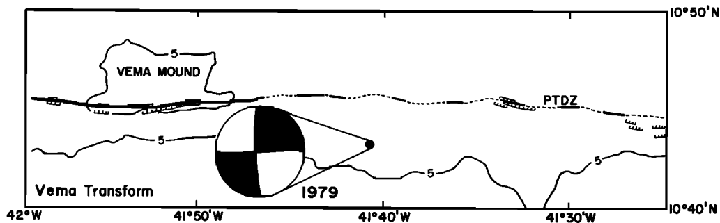
Fig. 8. Bathymetry and locus of the PTDZ for a portion of the central section of the Vema transform [from Macdonald et al. , 1986]. The 5-km isobath is shown. Also shown are the ISC epicenter (probably mislocated by about 5 km to the south) for the earthquake of August 25, 1979, and the focal mechanism of the primary subevent determined by body waveform inversion.
