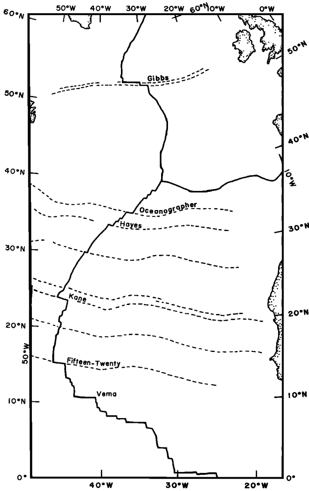
Fig. 1. Schematic map of the northern Mid-Atlantic Ridge, showing fracture zone traces (dashed lines) and the six transform faults considered in this study. Transverse Mercator projection, centered on the 40°W meridian. Adapted from Vogt [1986].
