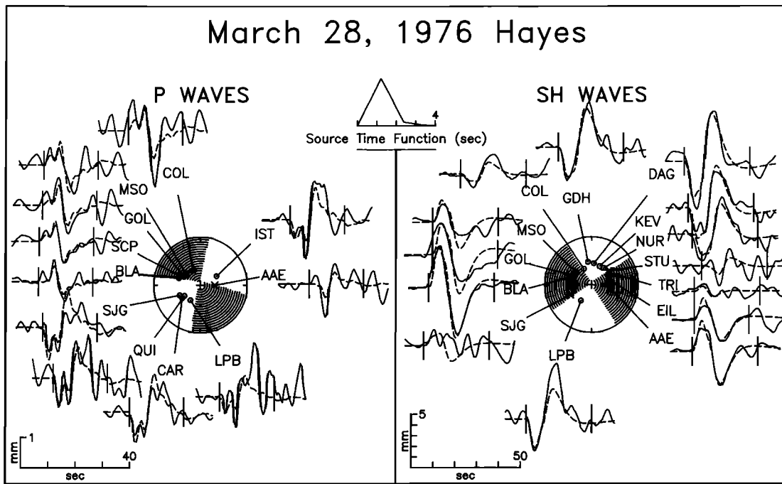
Fig. A4. Observed P and SH waves from the earthquake of March 28, 1976, on the Hayes transform compared with synthetic waveforms generated for the best fitting point source mechanism found from body waveform inversion. See Figure A1 for further explanation.
