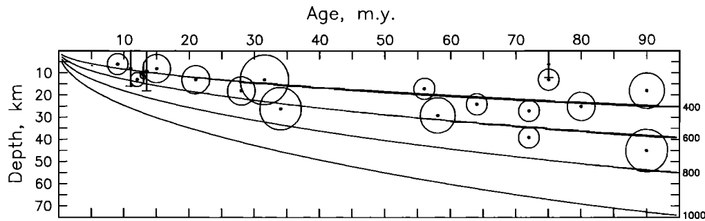
Fig. 13. Centroid depth versus lithosphere age for 18 oceanic intraplate earthquakes with strike-slip mechanisms. Two pairs of data points represent strike-slip subevents of earthquakes modelled as two or three point sources. Isotherms are from the plate cooling model of Parsons and Sclater [1977], with parameters identical to those assumed for the transform fault thermal model shown in Figures 11 and 12. Source parameters for these intraplate earthquakes were determined with the same body waveform inversion procedure as that used in this study. Fault radii were determined from the length of the source time function in the same manner as for the transform fault earthquakes (Appendix B). For three shallow events with apparent fault radii greater than their centroid depths, a rectangular fault geometry has been assumed, and the rupture is assumed to extend from the seafloor to twice the centroid depth.
