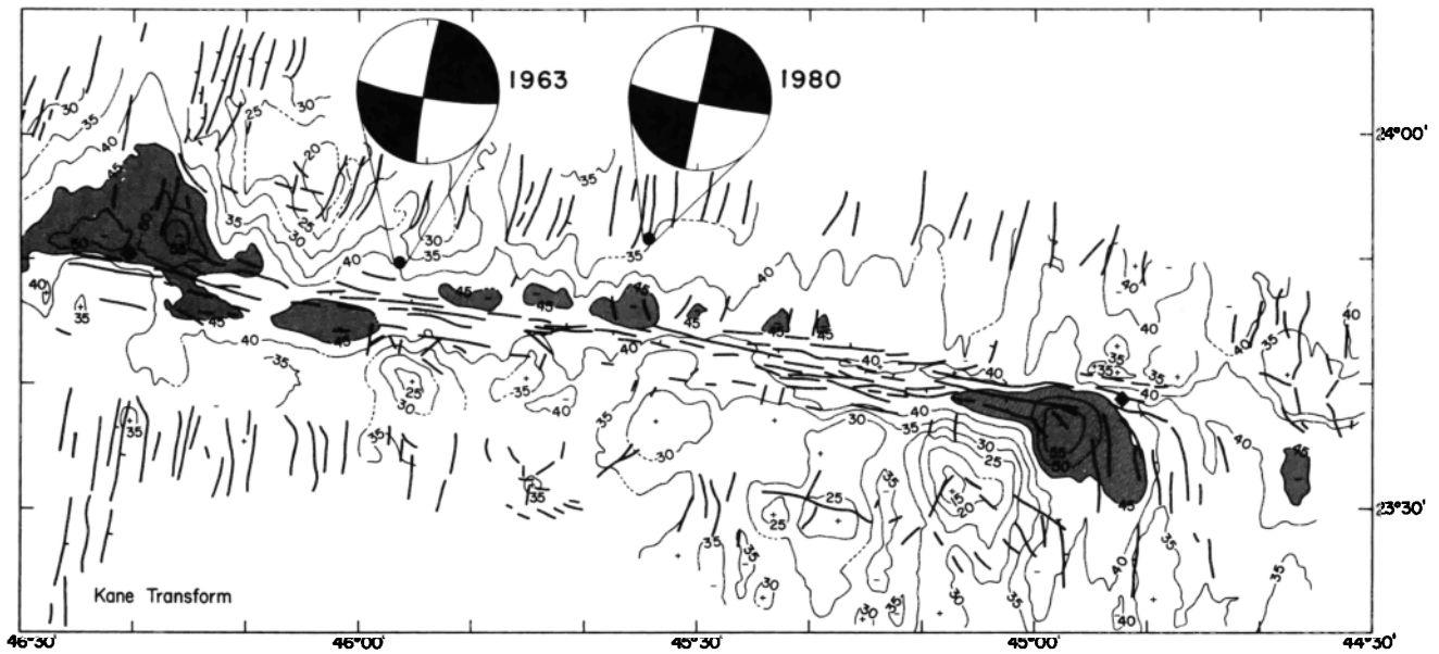
Fig. 5. Bathymetry and tectonic lineations of the Kane transform. Bathymetric contours, in hundreds of meters at 500-m intervals, are from a Sea Beam survey by Pockalny et al. [1988]. Areas deeper than 4500 m are shaded, and closed highs and lows are indicated by plus and minus signs. Tectonic lineations (heavy lines) are from a GLORIA side scan sonar survey reported by Searle [1986]. Positions of ridge-transform intersections are indicated by solid diamonds. Also shown are the ISC epicenter of the earthquake of March 26, 1980, and the relocated epicenter of the earthquake of May 19, 1963 (see text). Both epicenters are probably mislocated to the north by 5–15 km. Focal mechanisms, determined in this study by body waveform inversion, are shown for the primary subevent of each earthquake.
