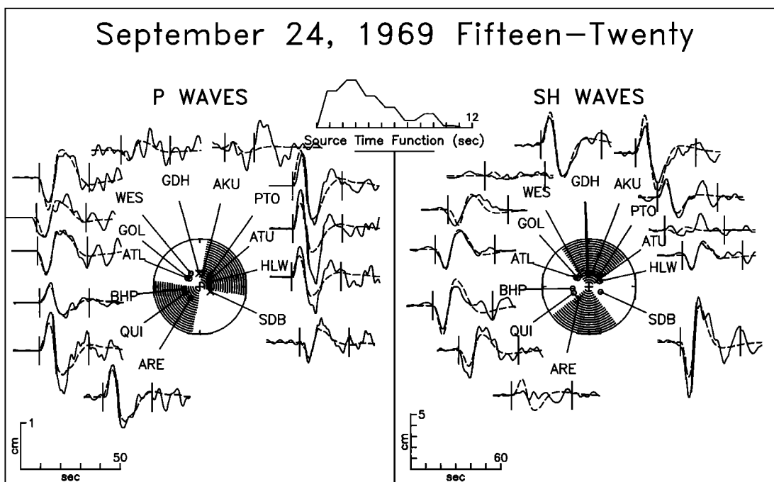
Fig. A7. Observed P and SH waves from the earthquake of September 24, 1969, on the 15°20' transform compared with synthetic waveforms generated for the best fitting point source mechanism found from body waveform inversion. See Figure A1 for further explanation.
