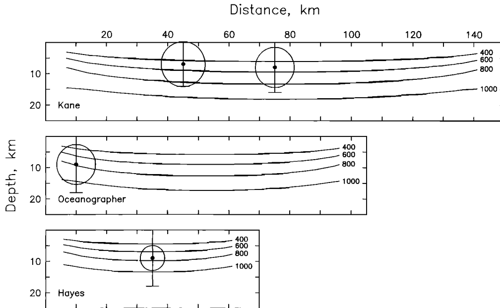
Fig. 12. Cross sections for Kane, Oceanographer, and Hayes transforms, showing the centroid depths and approximate depth extent of rupture during the earthquakes of this study and nominal isotherms (400°, 600°, 800°, and 1000°C) given by a simple thermal model (see text). See Figure 11 for further information.
