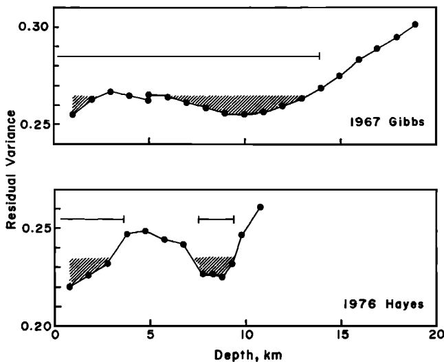
Fig. 10a. Residual variance as a function of centroid depth for two of the earthquakes in this study. The horizontal lines indicate the range in acceptable centroid depths at 90% confidence as given by the paired t test of Huang et al. [1986]. The shaded region indicates the range in acceptable centroid depths based on the 1% residual variance rule discussed in the text.
