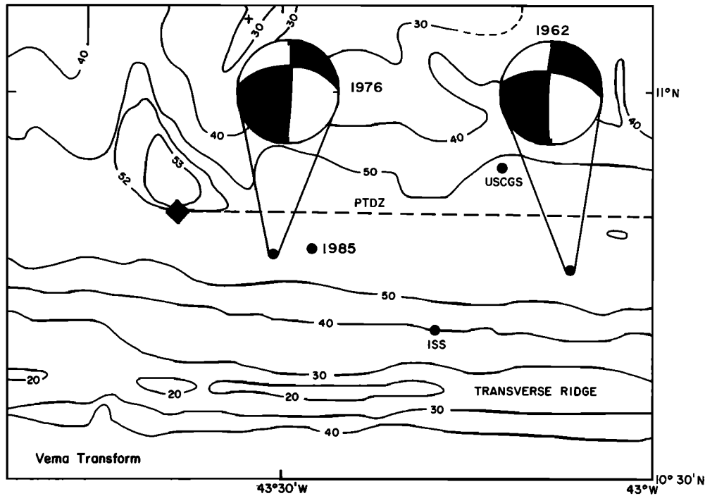
Fig. 7. Bathymetry of the western end of the Vema transform. bathymetric contours, in hundreds of meters, are from Louden et al. [1986]. The position of the PTDZ is from Rowlett and Forsyth [1984]. The position of the RTI is shown by a solid diamond. Also shown are the ISC epicenter for the earthquake of May 14, 1976, the epicenters determined for the earthquake of March 17, 1962 by the USCGS, ISS, and our relocation (see text), and the ISC epicenter for a large ( M_s 5.8) earthquake that occurred on January 10, 1985. All teleseismic epicenters are probably mislocated to the south by 5–10 km. Focal mechanisms were determined in this study by body waveform inversion.
