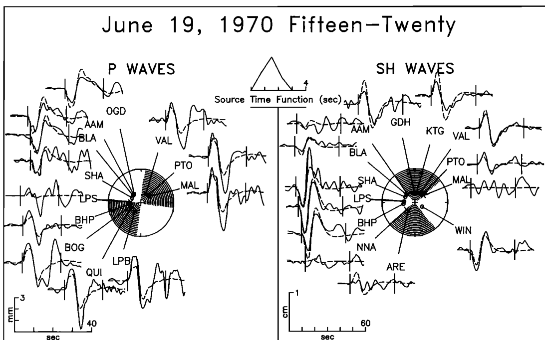
Fig. A8. Observed P and SH waves from the earthquake of June 19, 1970, on the 15°20' transform compared with synthetic waveforms generated for the best fitting point source mechanism found from body waveform inversion. See Figure A1 for further explanation.
