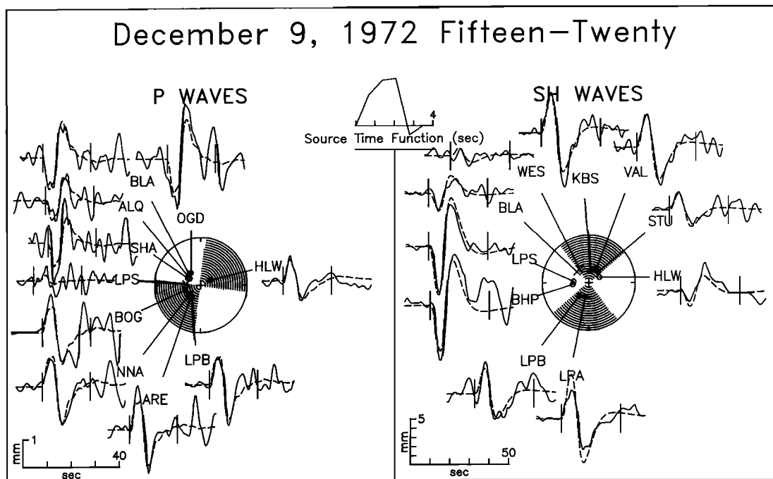
Fig. A9. Observed P and SH waves from the earthquake of December 9, 1972, on the 15^{\circ}20' transform compared with synthetic waveforms generated for the best fitting point source mechanism found from body waveform inversion. See Figure A1 for further explanation.
