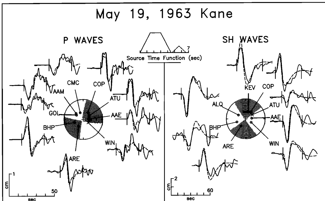
Fig. A5. Observed P and SH waves from the earthquake of May 19, 1963, on the Kane transform compared with synthetic waveforms generated for a source model with two point sources, the parameters of which were found from body waveform inversion. The radiation pattern of the largest subevent is shown. See Figure A1 for further explanation.
