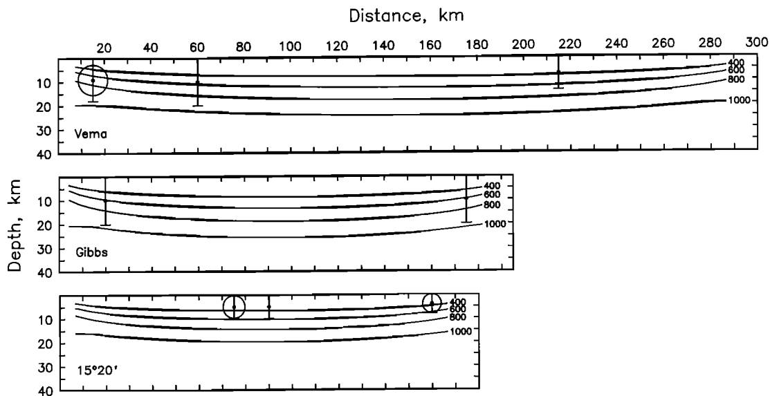
Fig. 11. Cross sections for the Vema, Gibbs, and 15°20' transforms, showing the centroid depths and approximate depth extent of rupture during the earthquakes of this study and nominal isotherms (400°, 600°, 800°, and 1000°C) given by a simple thermal model (see text). No vertical exaggeration. One estimate of the depth extent of rupture is from the seafloor to twice the centroid depth (vertical bars). For the smaller events of this study the depth extent of rupture has also been estimated from a simple circular fault model (circles).
