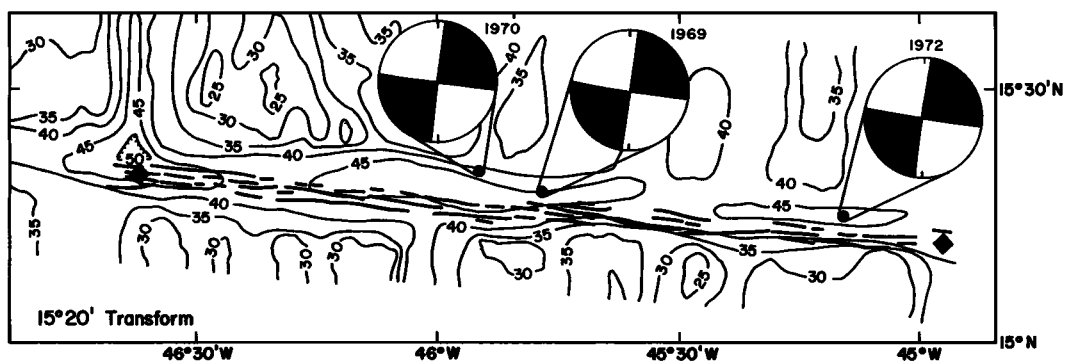
Fig. 6. Bathymetry and tectonic lineations of the 15^{\circ}20' transform. Bathymetric contours, in hundreds of meters at 500-m intervals, are from Searle [1986]. Tectonic lineations (heavy lines) are from a GLORIA side scan sonar survey [Searle, 1986]. Positions of ridge-transform intersections are indicated by solid diamonds. Also shown are the ISC epicenters (probably mislocated by about 5 km to the north) of the earthquakes of September 24, 1969, June 19, 1970, and December 9, 1972, along with the focal mechanisms determined in this study by body waveform inversion.
