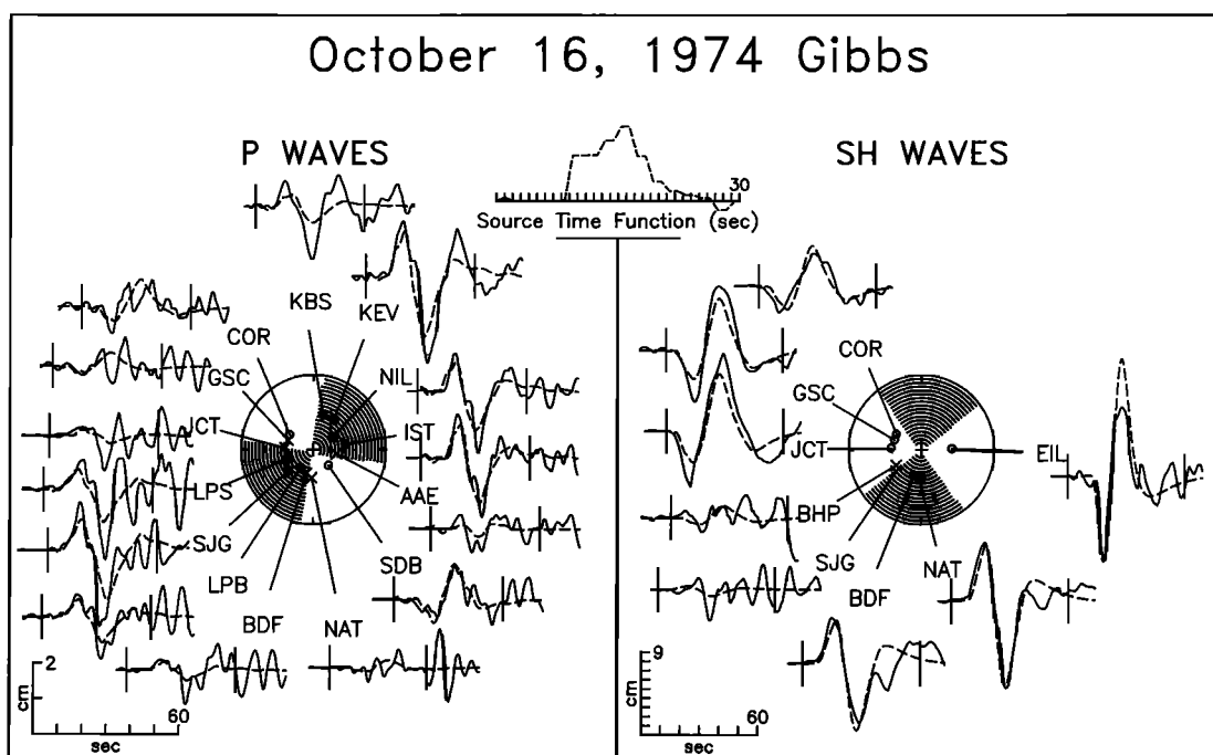
Fig. A2. Observed P and SH waves from the earthquake of October 16, 1974, on the Gibbs transform compared with synthetic waveforms generated for a source model with two point sources. The parameters of the first, small subevent were fixed in the inversion; the source parameters of the second subevent and its origin time and location relative to the first subevent were found from body waveform inversion. The radiation pattern of the largest subevent is shown. See Figure A1 for further explanation.
