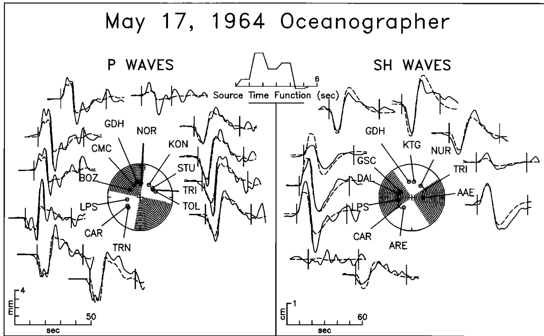
Fig. A3. Observed P and SH waves from the earthquake of May 17, 1964, on the Oceanographer transform compared with synthetic waveforms generated for the best fitting point source mechanism found from body waveform inversion. See Figure A1 for further explanation.
