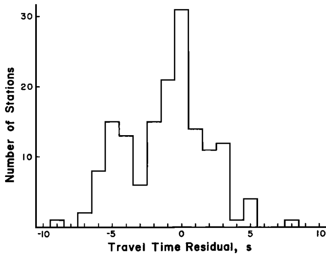
Fig. 9. Histogram of travel time residuals (observed-theoretical) for P waves from stations at epicentral distances less than 105^\circ from the Vema transform earthquake of March 17, 1962. The bimodal distribution shows the contribution to the reported arrival times of a small precursor which preceded the main rupture by about 5 s (see text).
