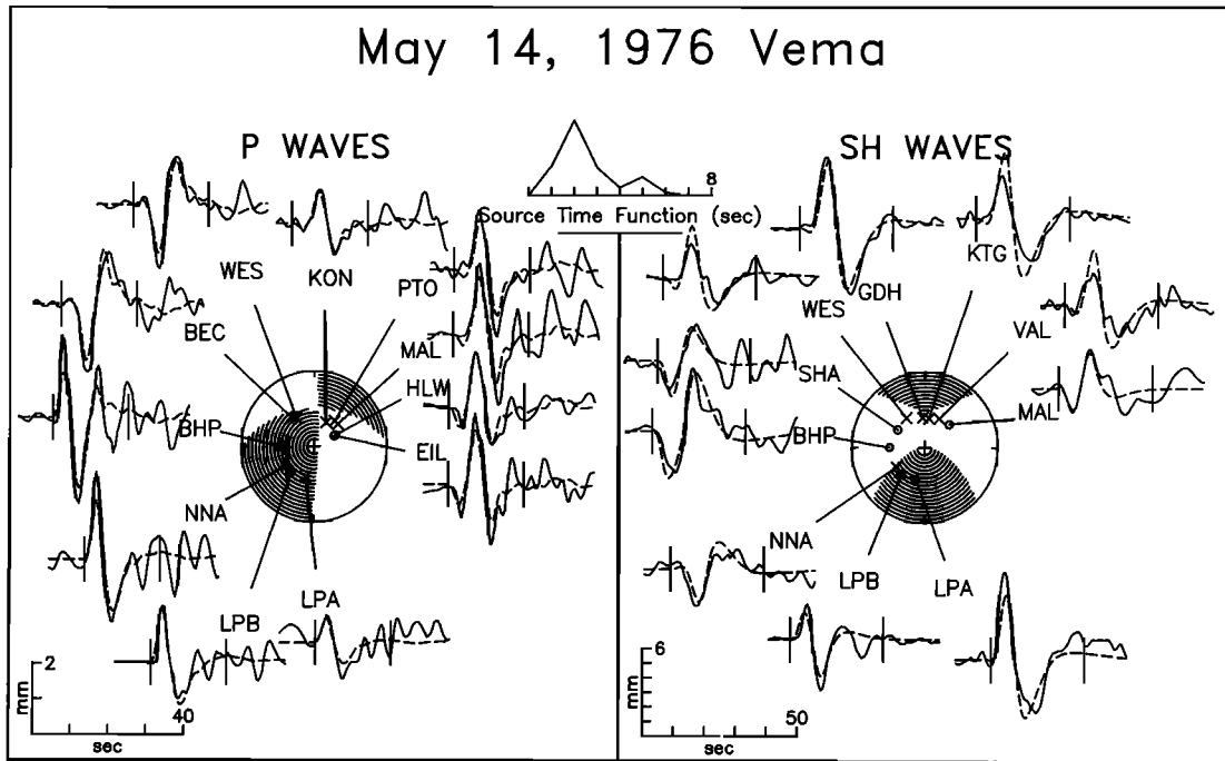
Fig. A11. Observed P and SH waves from the earthquake of May 14, 1976, on the Vema transform compared with synthetic waveforms generated for the best fitting point source mechanism found from body waveform inversion. See Figure A1 for further explanation.
