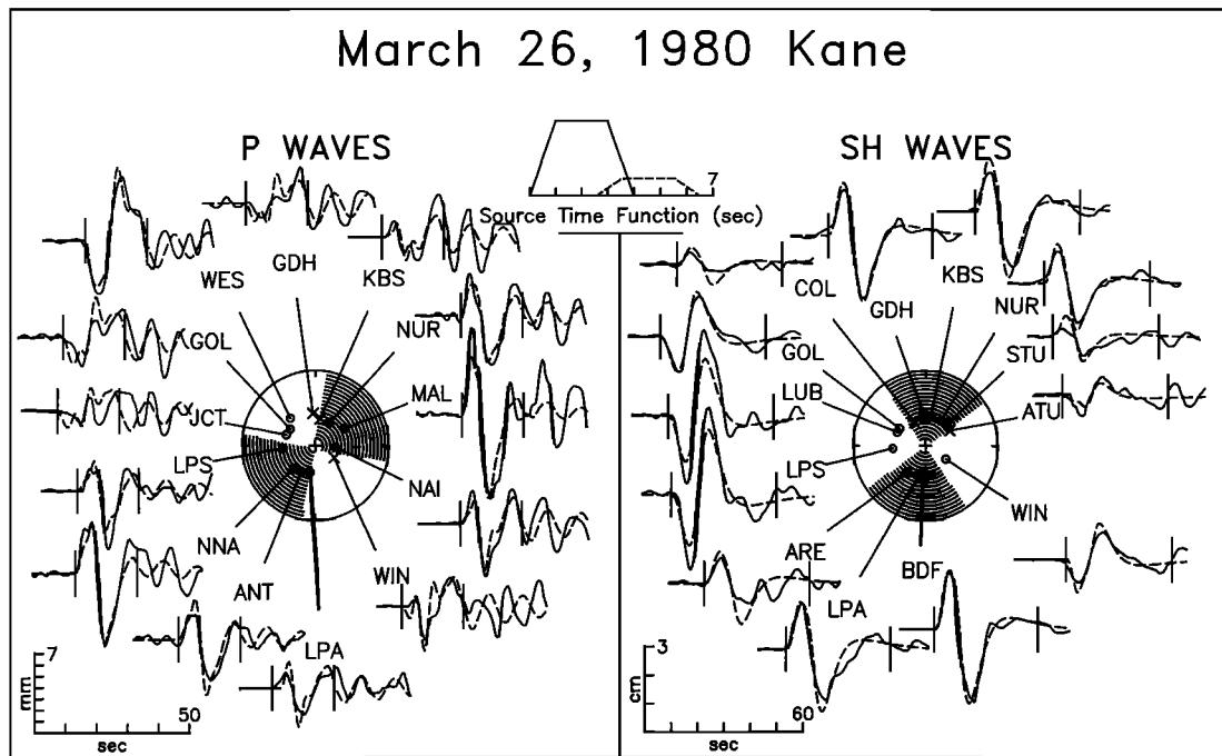
Fig. A6. Observed P and SH waves from the earthquake of March 26, 1980, on the Kane transform compared with synthetic waveforms generated for a source model with two point sources, the parameters of which were found from body waveform inversion. The radiation pattern of the largest subevent is shown. See Figure A1 for further explanation.
