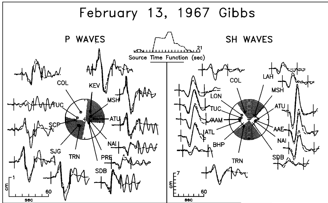
Fig. A1. Observed (solid curves) long-period P and SH waves from the earthquake of February 13, 1967, on the Gibbs transform compared with synthetic waveforms (dashed curves) generated for a source model with two point sources. The parameters of the first, small subevent were fixed in the inversion; the source parameters of the second subevent and its origin time and location relative to the first subevent were found from body waveform inversion. The radiation pattern of the largest subevent is shown. P and SH radiation patterns are shown on the lower focal hemisphere (equal-area projection). All amplitudes are normalized to an epicentral distance of 40^\circ and a WWSSN instrument magnification of 1500; the amplitude scales correspond to the waveforms that would be observed on an original seismogram from such an instrument. The two vertical lines delimit the portion of each time series used in the inversion. For SH waves, compression corresponds to positive motion as defined by Aki and Richards [1980]. Full names and locations of all stations are given by Poppe et al. [1978].
