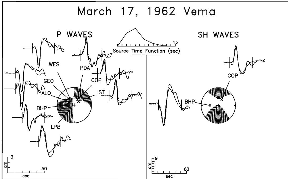
Fig. A10. Observed P and SH waves from the earthquake of March 17, 1962, on the Vema transform compared with synthetic waveforms generated for the best fitting point source mechanism found from body waveform inversion. See Figure A1 for further explanation.
