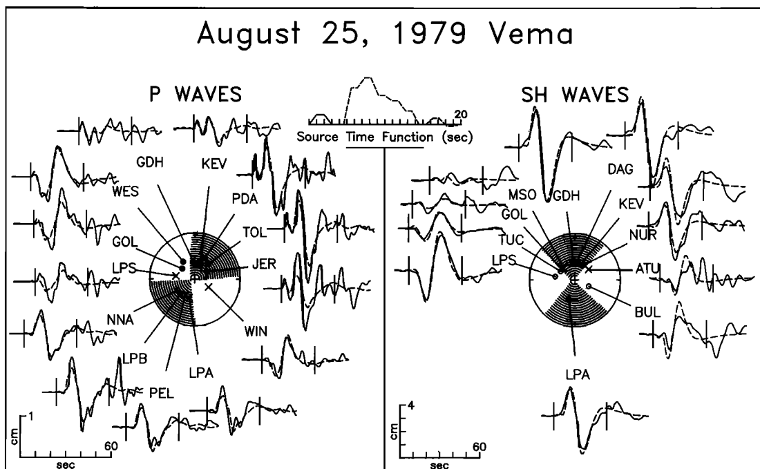
Fig. A12. Observed P and SH waves from the earthquake of August 25, 1979, on the Vema transform compared with synthetic waveforms generated for a source model with two point sources. The parameters of the first, small subevent were fixed in the inversion; the source parameters of the second subevent and its origin time and location relative to the first subevent were found from body waveform inversion. The radiation pattern of the largest subevent is shown. See Figure A1 for further explanation.
