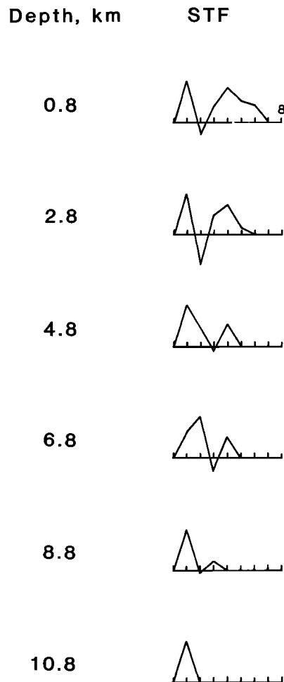
Fig. 10b. Best fitting source time function (STF) for the 1976 Hayes transform earthquake, obtained in a series of waveform inversions with the centroid depth constrained at the indicated values. The double-peaked character at shallow depths yields waveforms that mimic depth phases.
